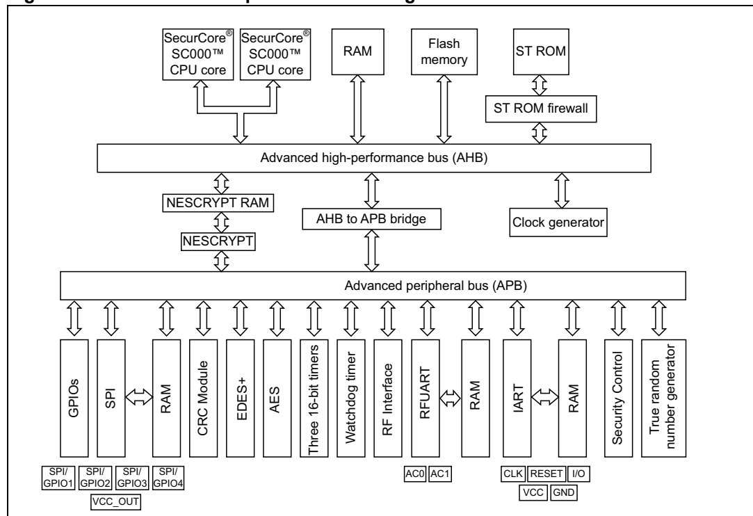
Figure 1. ST31N600 A01 platform block diagram
